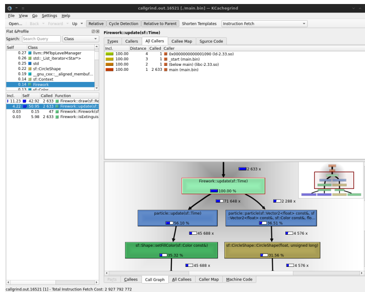
Figure 436: Using Valgrind's Callgrind tool and Kcachegrind we can see what is bogging down our game
